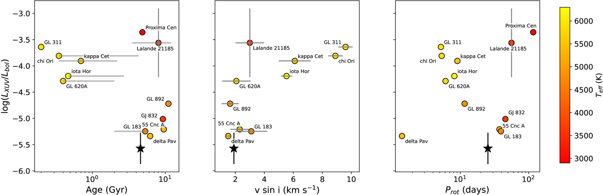
Figure 7. from Sarah Peacock et al 2026 Astrophys. J. 1009 doi:10.3847/1538-4357/aea076 https://dx.doi.org/10.3847/1538-4357/aea076 © 2026. The Author(s). Published by the American Astronomical Society.
