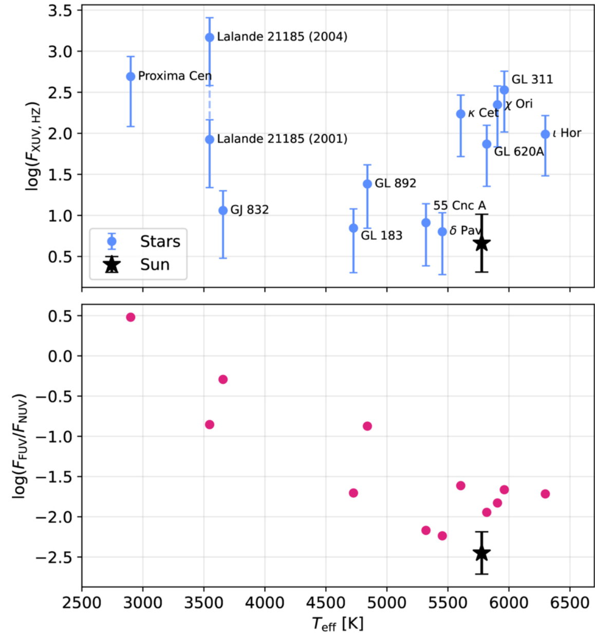
Figure 5. from Sarah Peacock et al 2026 Astrophys. J. 1009 doi:10.3847/1538-4357/aea076 https://dx.doi.org/10.3847/1538-4357/aea076 © 2026. The Author(s). Published by the American Astronomical Society.
