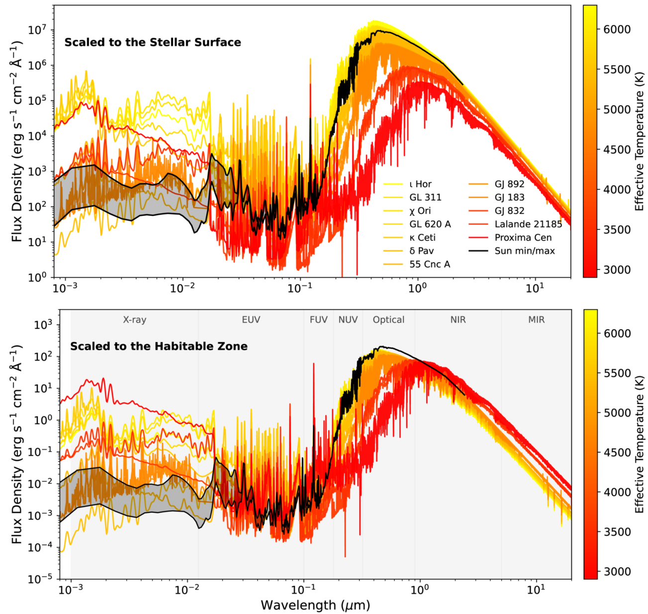
Figure 3. from Sarah Peacock et al 2026 Astrophys. J. 1009 doi:10.3847/1538-4357/aea076 https://dx.doi.org/10.3847/1538-4357/aea076 © 2026. The Author(s). Published by the American Astronomical Society.
