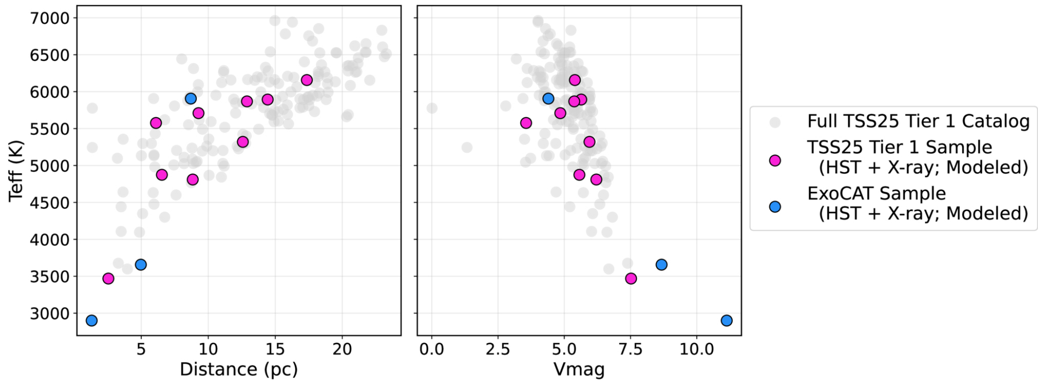
Figure 1. from Sarah Peacock et al 2026 Astrophys. J. 1009 doi:10.3847/1538-4357/aea076 https://dx.doi.org/10.3847/1538-4357/aea076 © 2026. The Author(s). Published by the American Astronomical Society.
