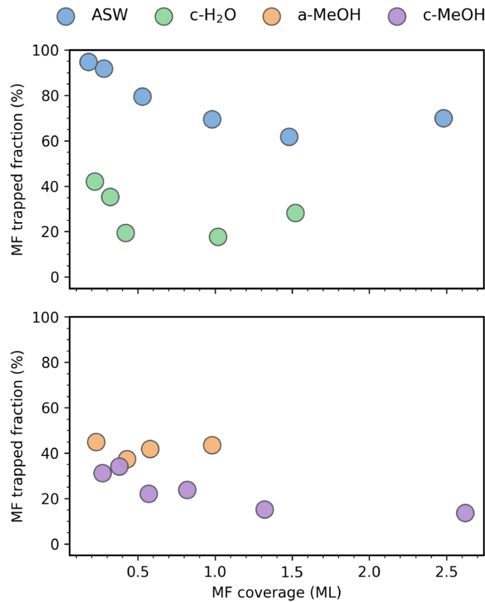
Figure 7. from Rachel E. Gross et al 2026 Astrophys. J. 1010 doi:10.3847/1538-4357/ae9fee https://dx.doi.org/10.3847/1538-4357/ae9fee © 2026. The Author(s). Published by the American Astronomical Society.
