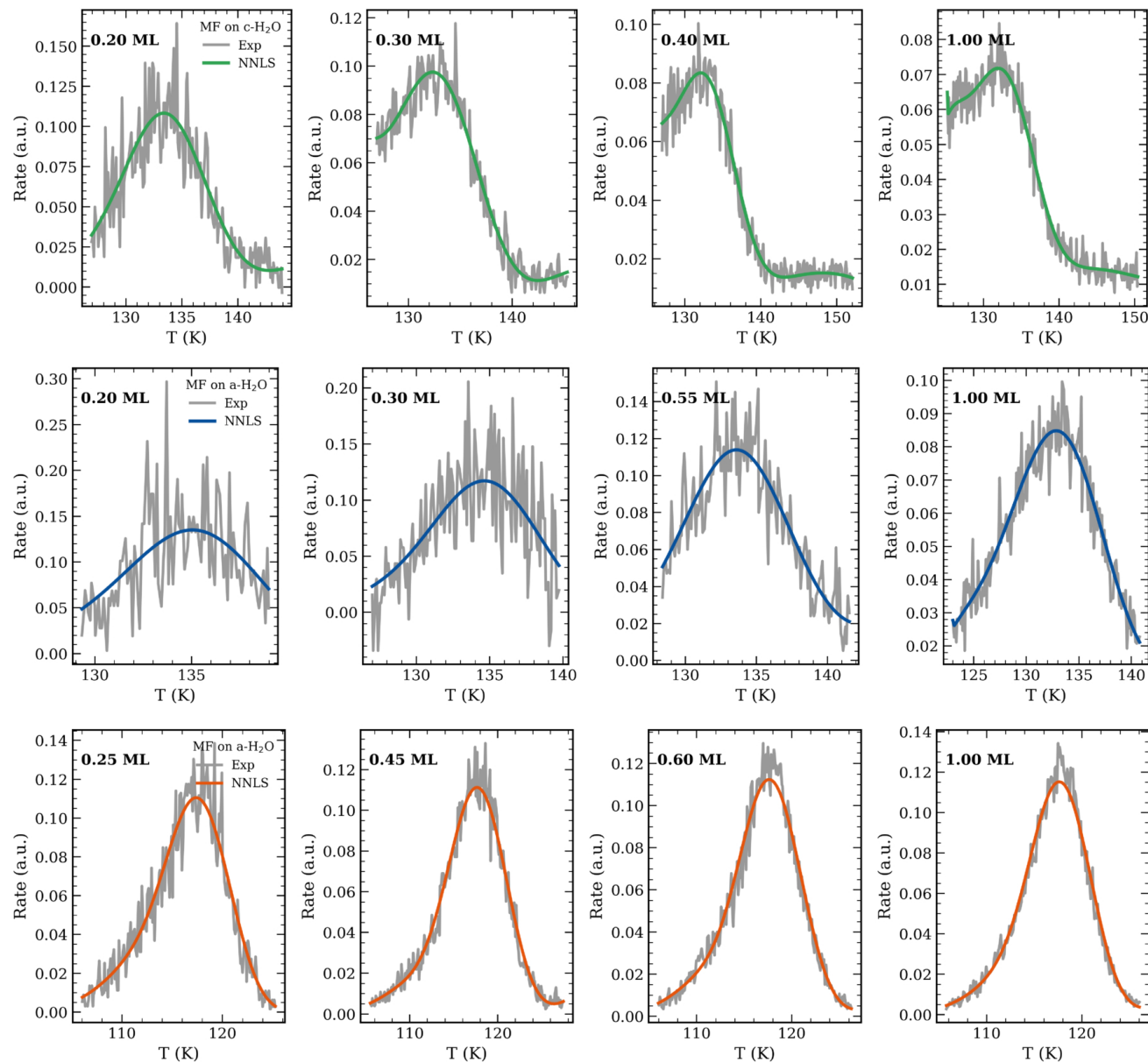
Figure F1. from Rachel E. Gross et al 2026 Astrophys. J. 1010 doi:10.3847/1538-4357/ae9fee https://dx.doi.org/10.3847/1538-4357/ae9fee © 2026. The Author(s). Published by the American Astronomical Society.
