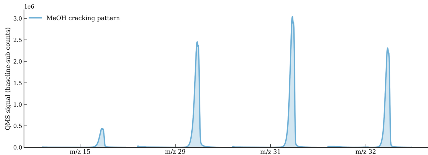
(b) MeOH cracking pattern
