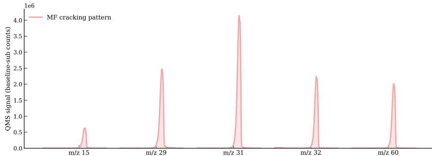
(a) MF cracking pattern
