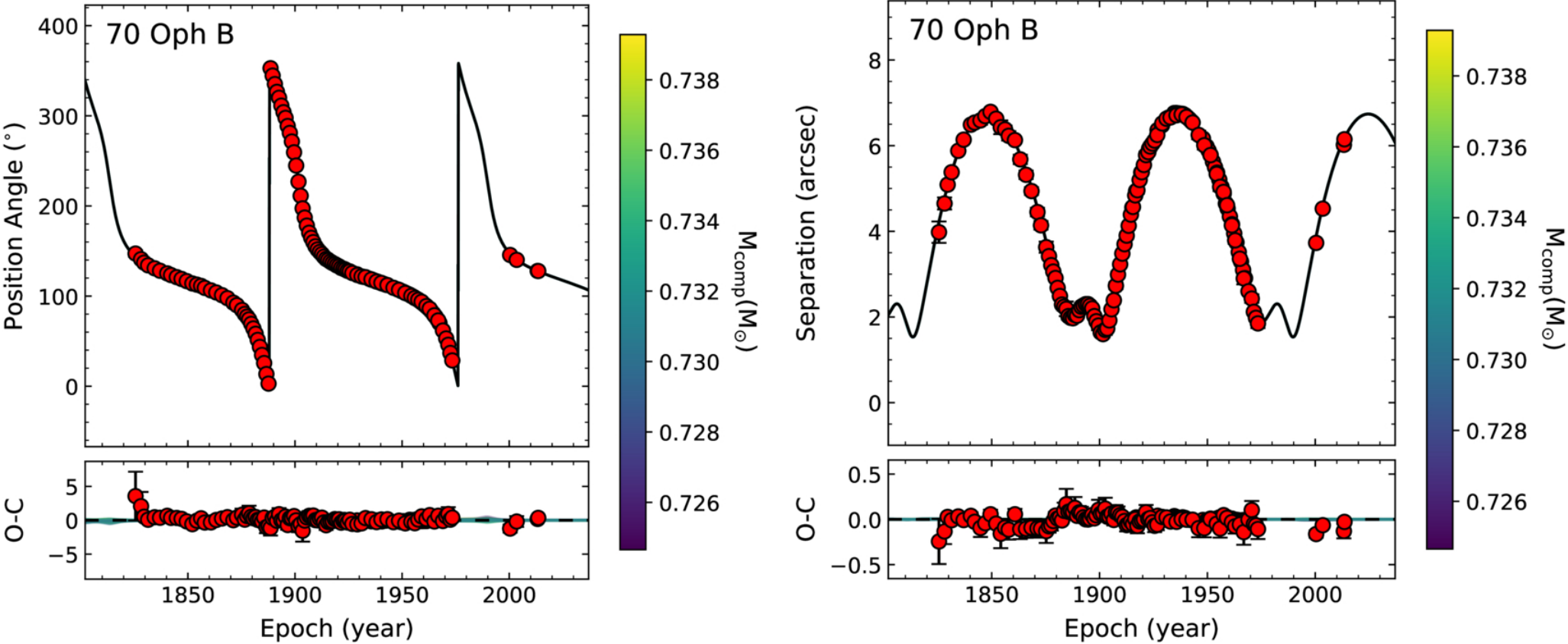
Figure 3. from Yiting Li et al 2026 Astrophys. J. 1009 doi:10.3847/1538-4357/ae9f52 https://dx.doi.org/10.3847/1538-4357/ae9f52 © 2026. The Author(s). Published by the American Astronomical Society.
