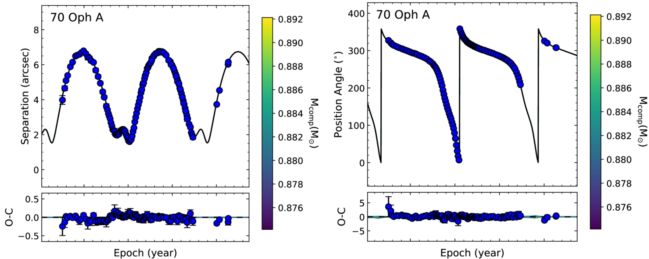
Figure A2. from Yiting Li et al 2026 Astrophys. J. 1009 doi:10.3847/1538-4357/ae9f52 https://dx.doi.org/10.3847/1538-4357/ae9f52 © 2026. The Author(s). Published by the American Astronomical Society.
