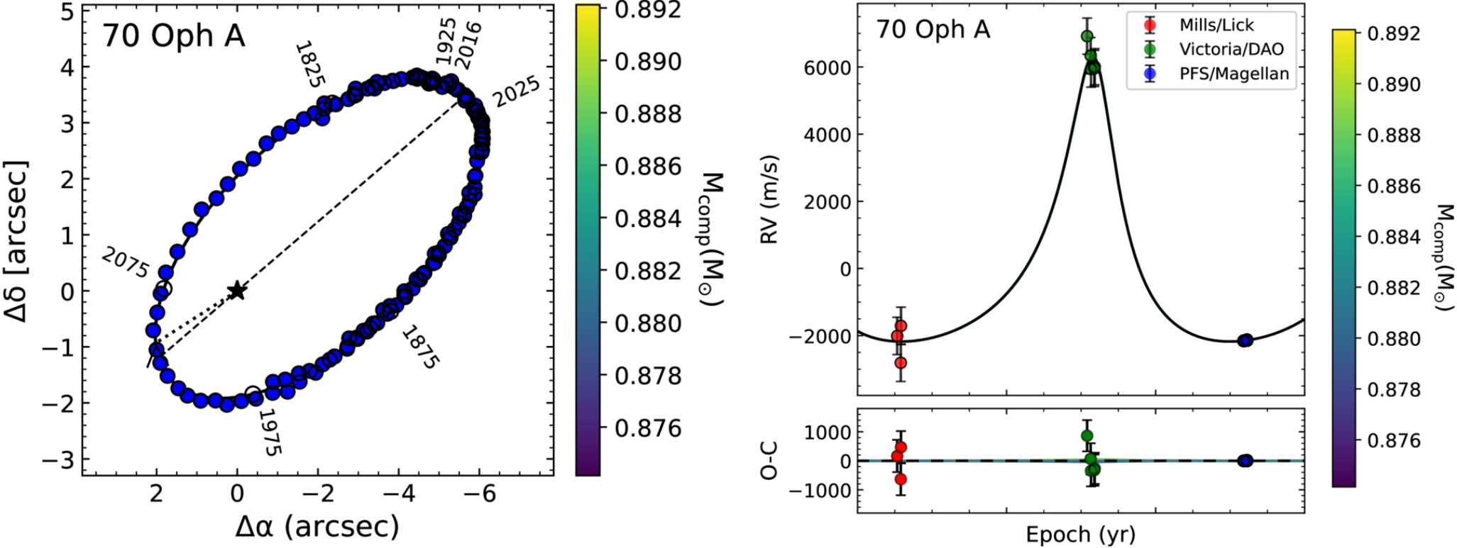
Figure A1. from Yiting Li et al 2026 Astrophys. J. 1009 doi:10.3847/1538-4357/ae9f52 https://dx.doi.org/10.3847/1538-4357/ae9f52 © 2026. The Author(s). Published by the American Astronomical Society.
