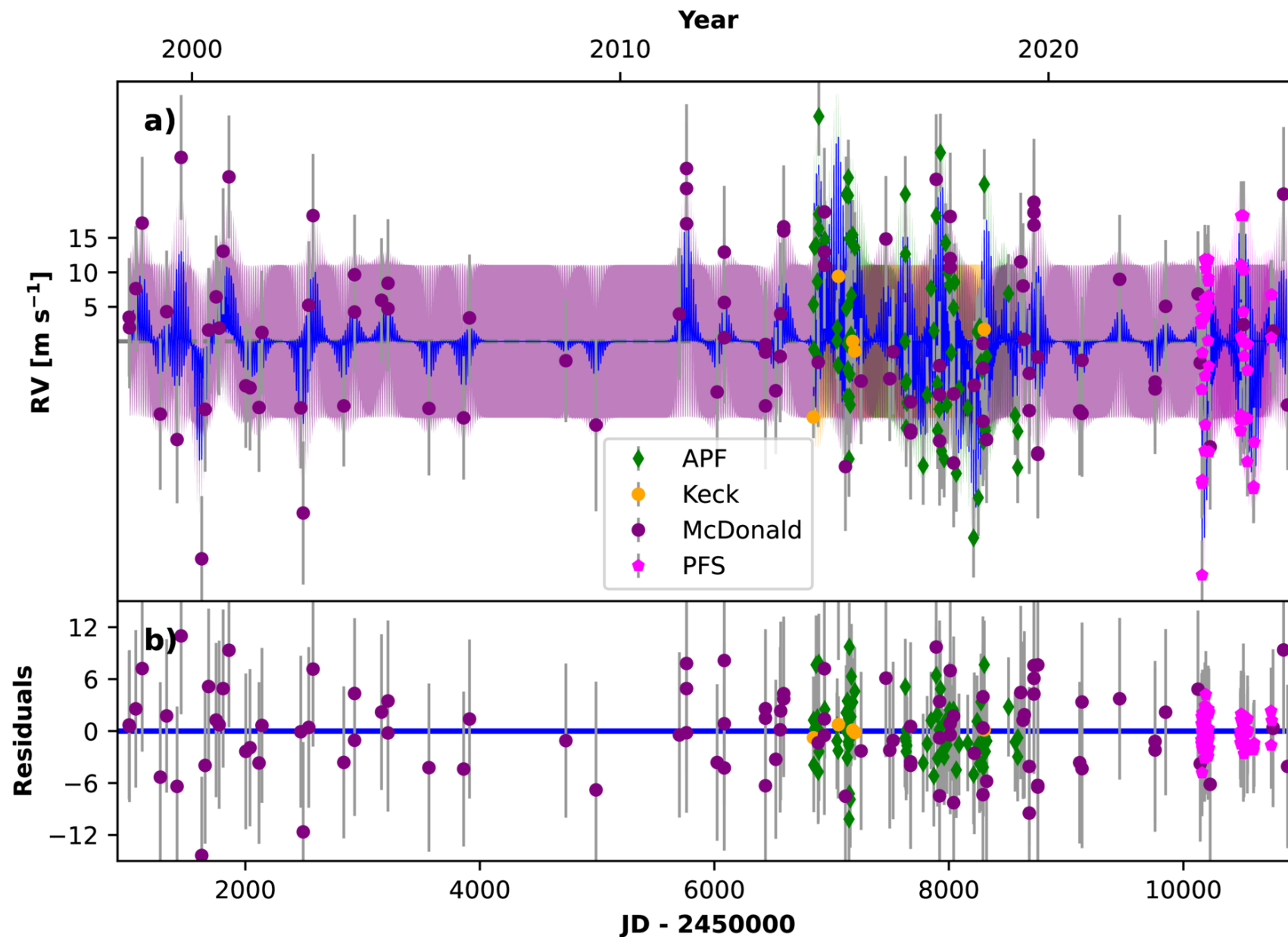
Figure 10. from Yiting Li et al 2026 Astrophys. J. 1009 doi:10.3847/1538-4357/ae9f52 https://dx.doi.org/10.3847/1538-4357/ae9f52 © 2026. The Author(s). Published by the American Astronomical Society.
