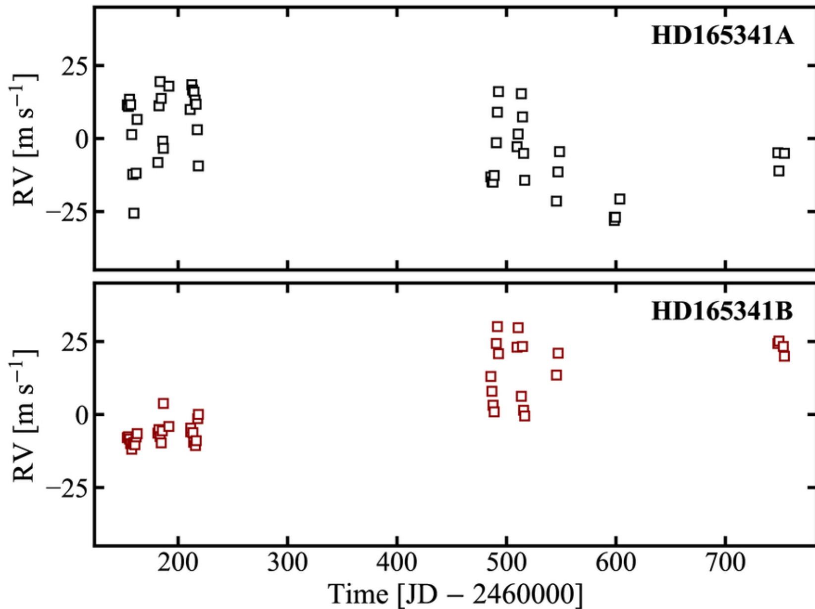
Figure 1. from Yiting Li et al 2026 Astrophys. J. 1009 doi:10.3847/1538-4357/ae9f52 https://dx.doi.org/10.3847/1538-4357/ae9f52 © 2026. The Author(s). Published by the American Astronomical Society.
