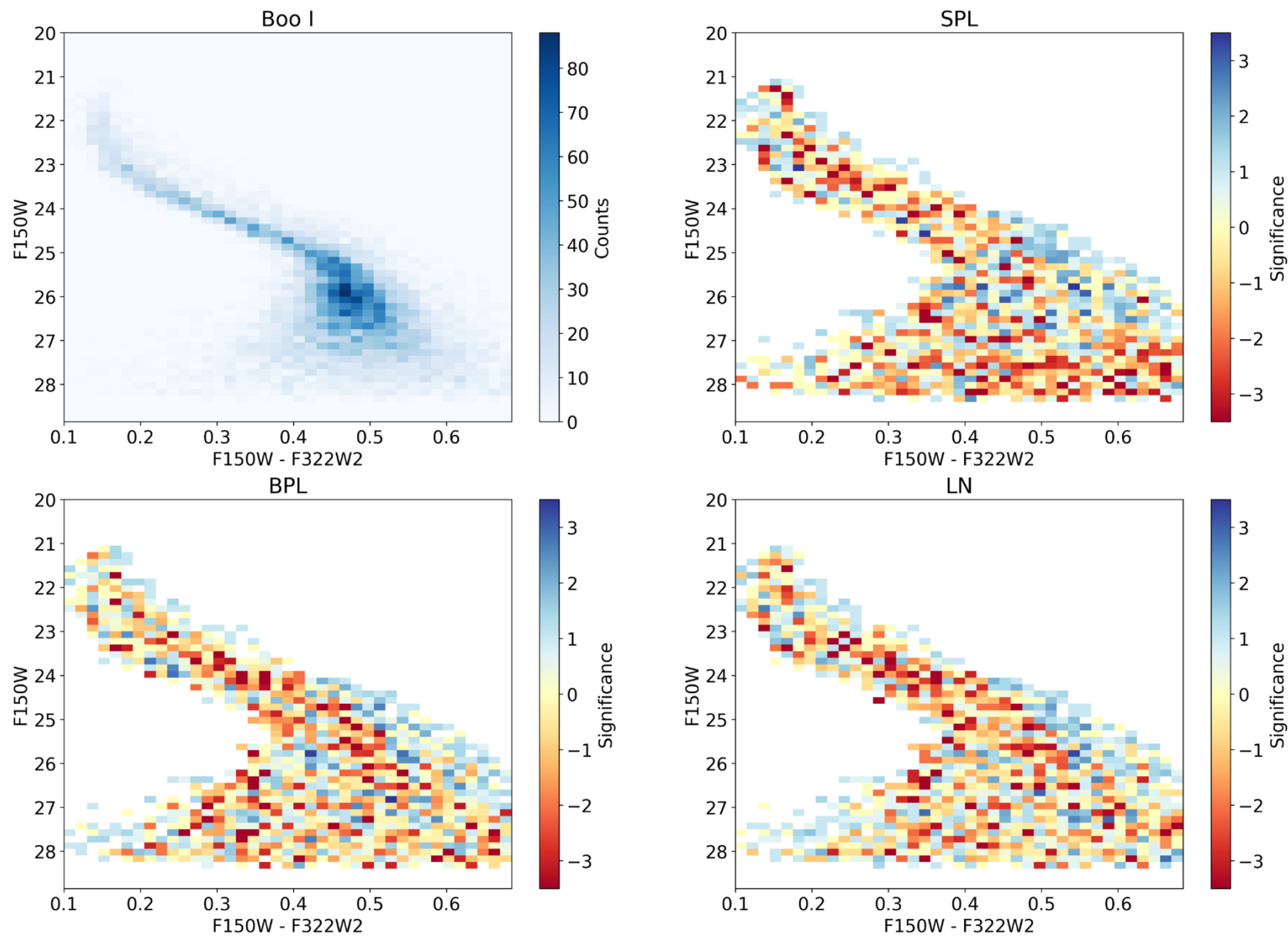
Figure 8. from Keyi Ding et al 2026 Astrophys. J. 1009 doi:10.3847/1538-4357/ae9f3e https://dx.doi.org/10.3847/1538-4357/ae9f3e © 2026. The Author(s). Published by the American Astronomical Society.
