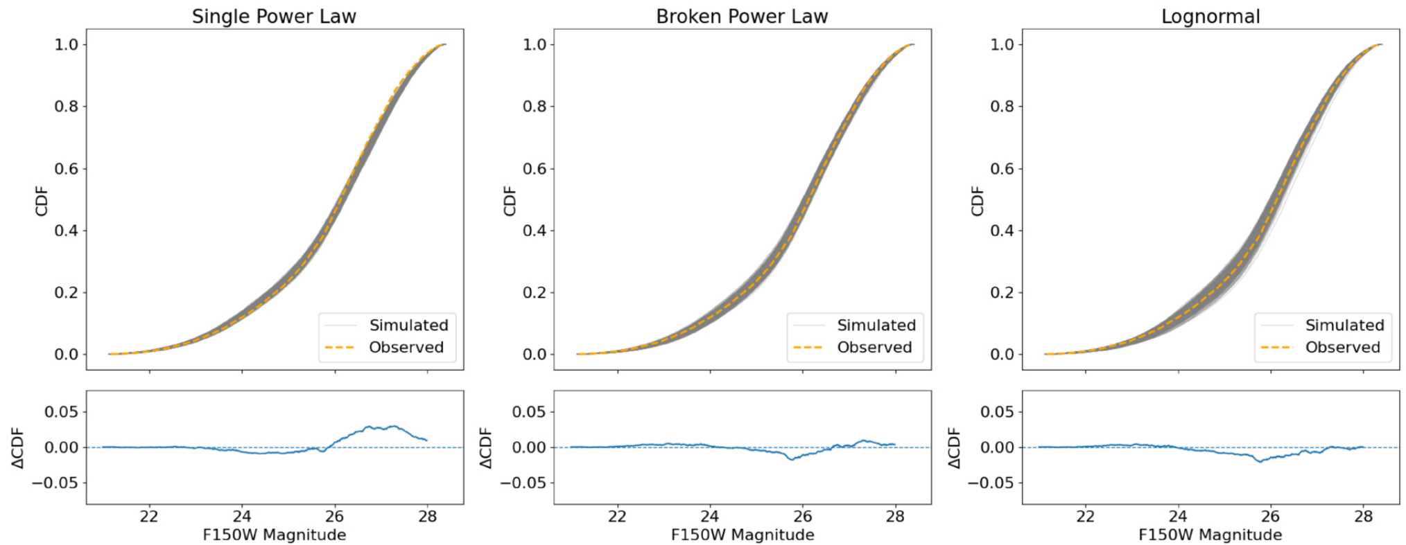
Figure 7. from Keyi Ding et al 2026 Astrophys. J. 1009 doi:10.3847/1538-4357/ae9f3e https://dx.doi.org/10.3847/1538-4357/ae9f3e © 2026. The Author(s). Published by the American Astronomical Society.
