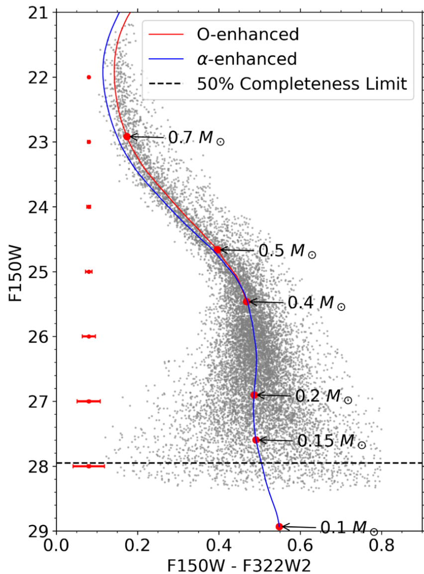
Figure 4. from Keyi Ding et al 2026 Astrophys. J. 1009 doi:10.3847/1538-4357/ae9f3e https://dx.doi.org/10.3847/1538-4357/ae9f3e © 2026. The Author(s). Published by the American Astronomical Society.
