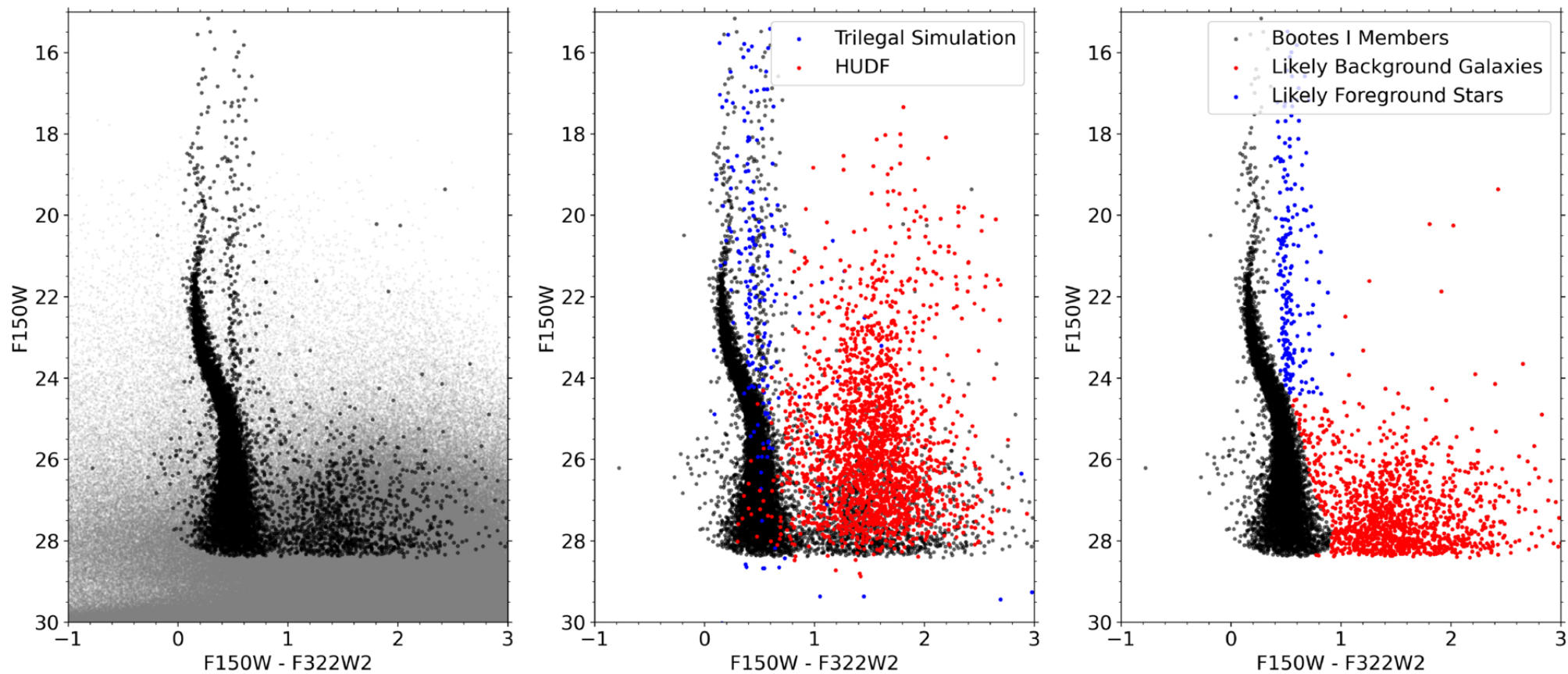
Figure 2. from Keyi Ding et al 2026 Astrophys. J. 1009 doi:10.3847/1538-4357/ae9f3e https://dx.doi.org/10.3847/1538-4357/ae9f3e © 2026. The Author(s). Published by the American Astronomical Society.
