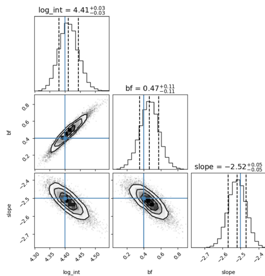
(a) Single power-law
