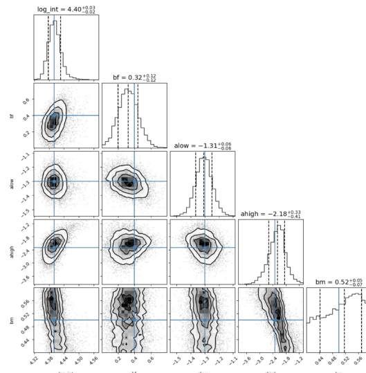
(b) Broken power-law
