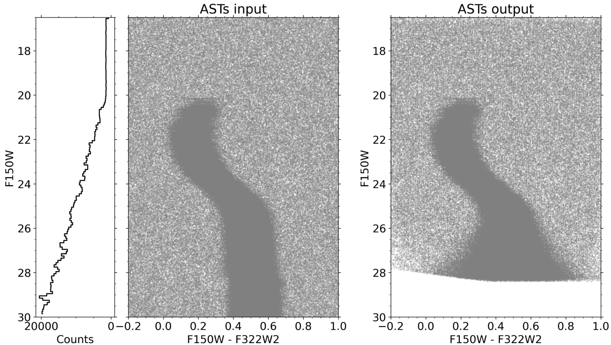
Figure B1. from Keyi Ding et al 2026 Astrophys. J. 1009 doi:10.3847/1538-4357/ae9f3e https://dx.doi.org/10.3847/1538-4357/ae9f3e © 2026. The Author(s). Published by the American Astronomical Society.
