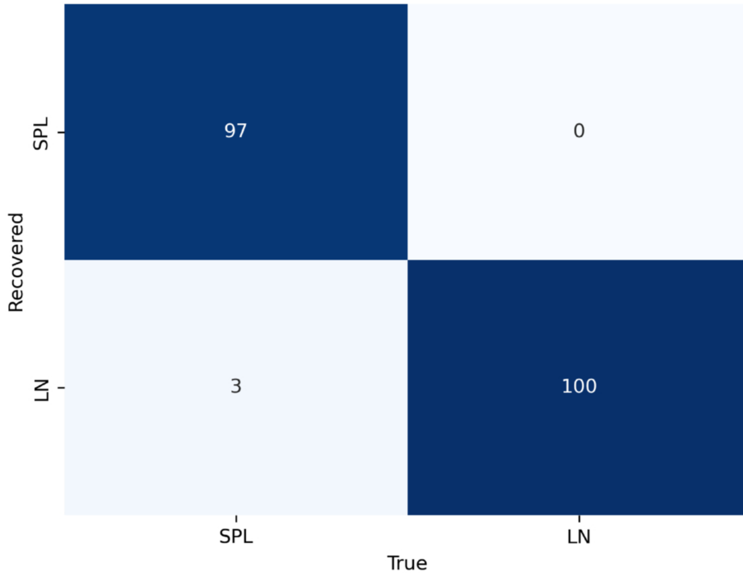
Figure 10. from Keyi Ding et al 2026 Astrophys. J. 1009 doi:10.3847/1538-4357/ae9f3e https://dx.doi.org/10.3847/1538-4357/ae9f3e © 2026. The Author(s). Published by the American Astronomical Society.
