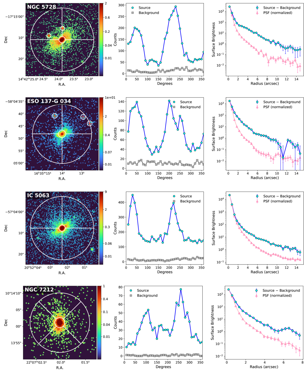
Figure 7. from R. Middei et al 2026 Astrophys. J. 1010 doi:10.3847/1538-4357/ae9eb9 https://dx.doi.org/10.3847/1538-4357/ae9eb9 © 2026. The Author(s). Published by the American Astronomical Society.
