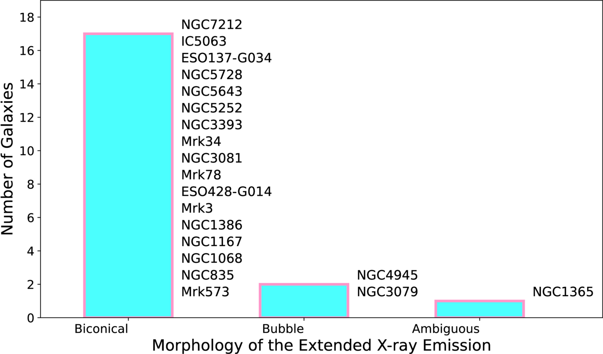
Figure 2. from R. Middei et al 2026 Astrophys. J. 1010 doi:10.3847/1538-4357/ae9eb9 https://dx.doi.org/10.3847/1538-4357/ae9eb9 © 2026. The Author(s). Published by the American Astronomical Society.
