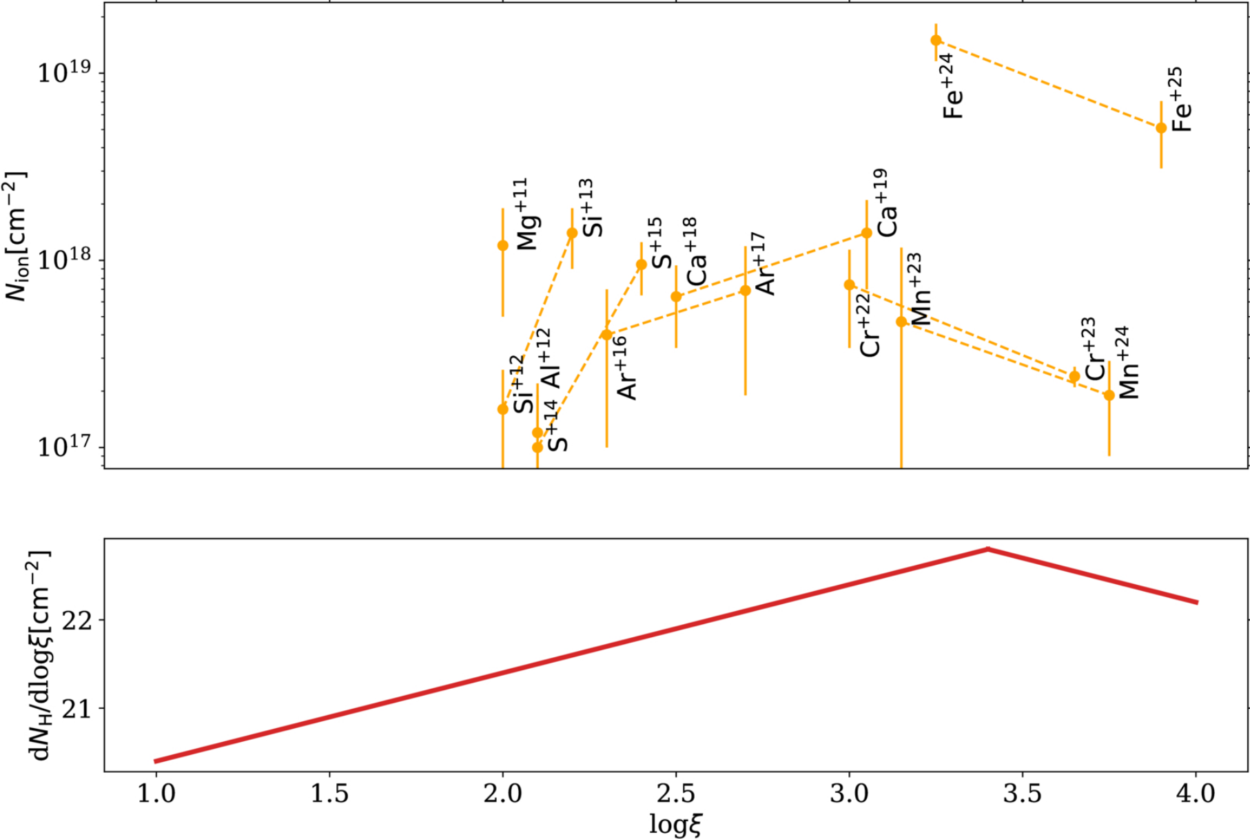
Figure 3. from Noa Keshet et al 2026 Astrophys. J. 1010 doi:10.3847/1538-4357/ae9d59 https://dx.doi.org/10.3847/1538-4357/ae9d59 © 2026. The Author(s). Published by the American Astronomical Society.
