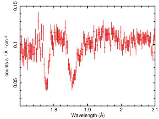
Figure 2. from Noa Keshet et al 2026 Astrophys. J. 1010 doi:10.3847/1538-4357/ae9d59 https://dx.doi.org/10.3847/1538-4357/ae9d59 © 2026. The Author(s). Published by the American Astronomical Society.
