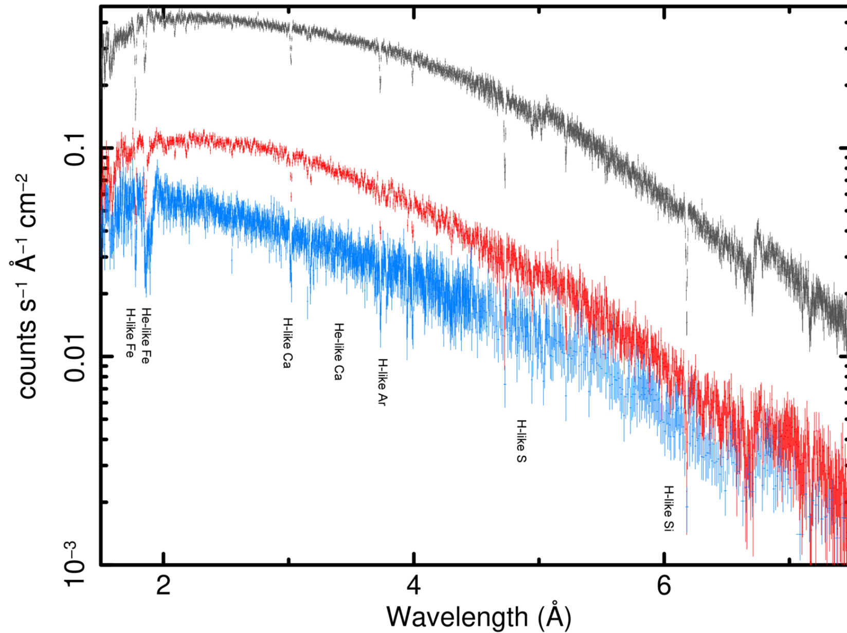
Figure 1. from Noa Keshet et al 2026 Astrophys. J. 1010 doi:10.3847/1538-4357/ae9d59 https://dx.doi.org/10.3847/1538-4357/ae9d59 © 2026. The Author(s). Published by the American Astronomical Society.
