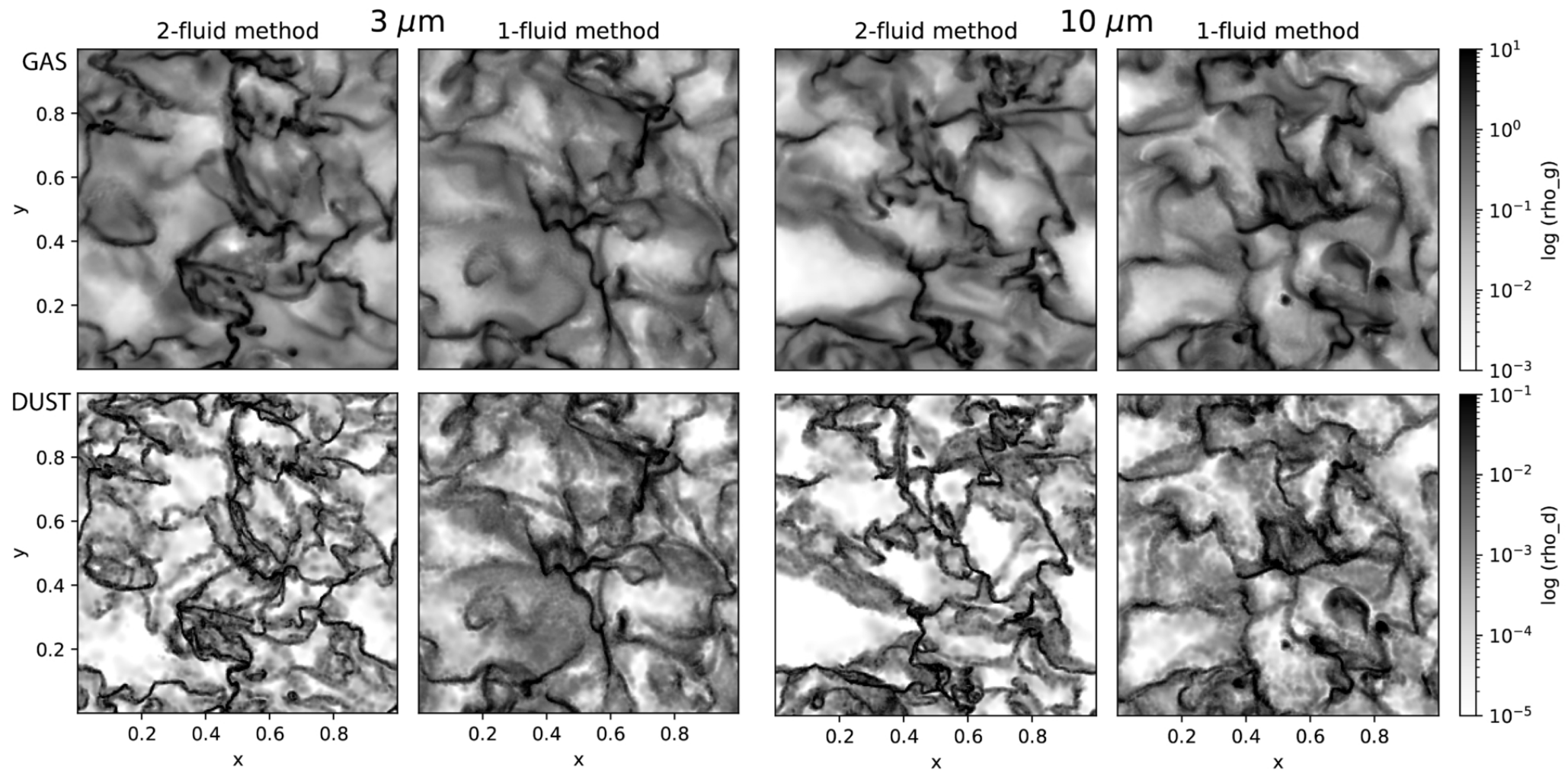
Figure 6. from Narges Vadood and Terrence S. Tricco 2026 Astrophys. J. 1009 doi:10.3847/1538-4357/ae9cb9 https://dx.doi.org/10.3847/1538-4357/ae9cb9 © 2026. The Author(s). Published by the American Astronomical Society.
