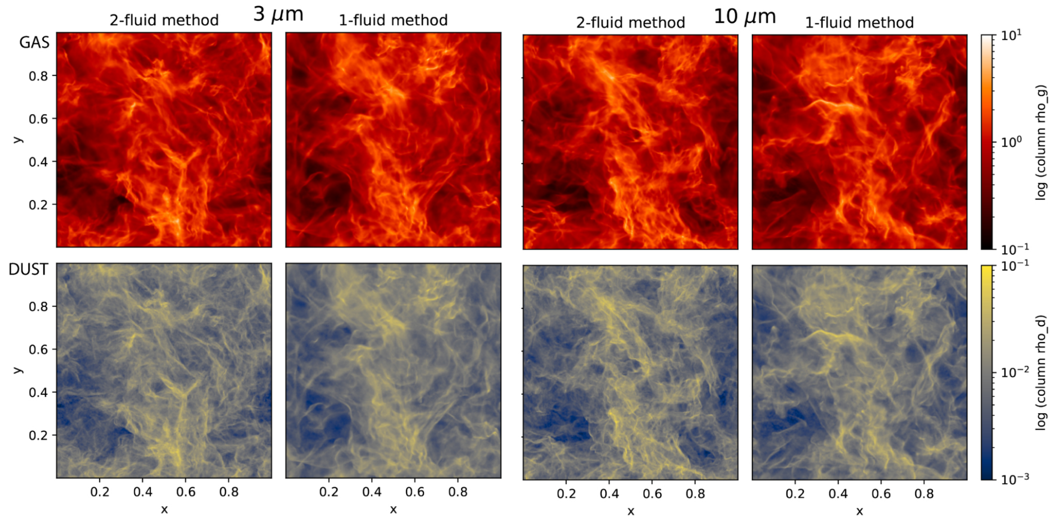
Figure 5. from Narges Vadood and Terrence S. Tricco 2026 Astrophys. J. 1009 doi:10.3847/1538-4357/ae9cb9 https://dx.doi.org/10.3847/1538-4357/ae9cb9 © 2026. The Author(s). Published by the American Astronomical Society.
