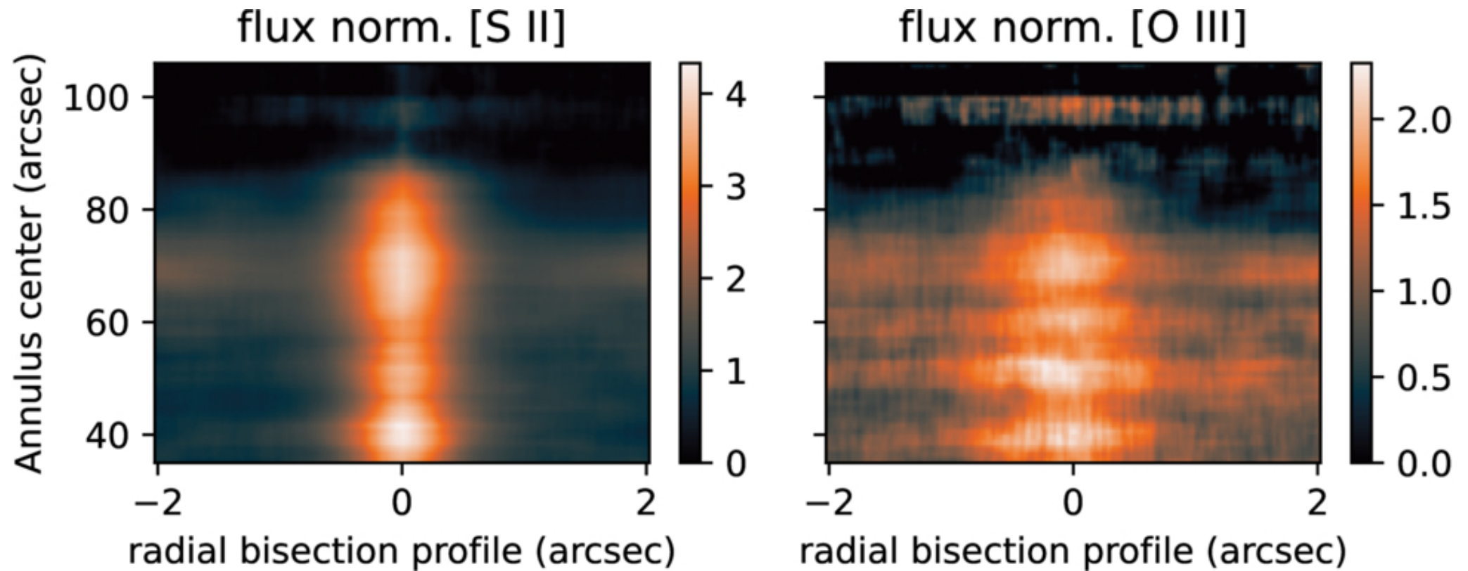
Figure 6. from Tim Cunningham et al 2026 Astrophys. J. 1010 doi:10.3847/1538-4357/ae9cb2 https://dx.doi.org/10.3847/1538-4357/ae9cb2 © 2026. The Author(s). Published by the American Astronomical Society.
