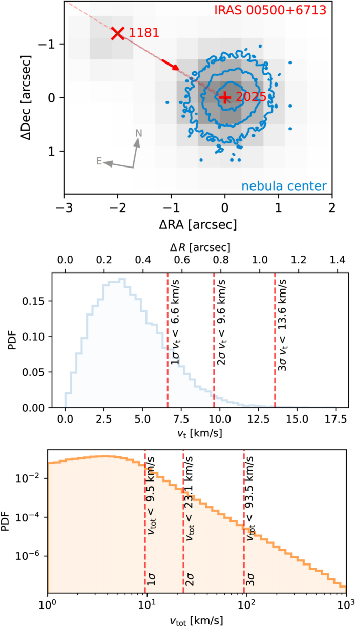
Figure 4. from Tim Cunningham et al 2026 Astrophys. J. 1010 doi:10.3847/1538-4357/ae9cb2 https://dx.doi.org/10.3847/1538-4357/ae9cb2 © 2026. The Author(s). Published by the American Astronomical Society.
