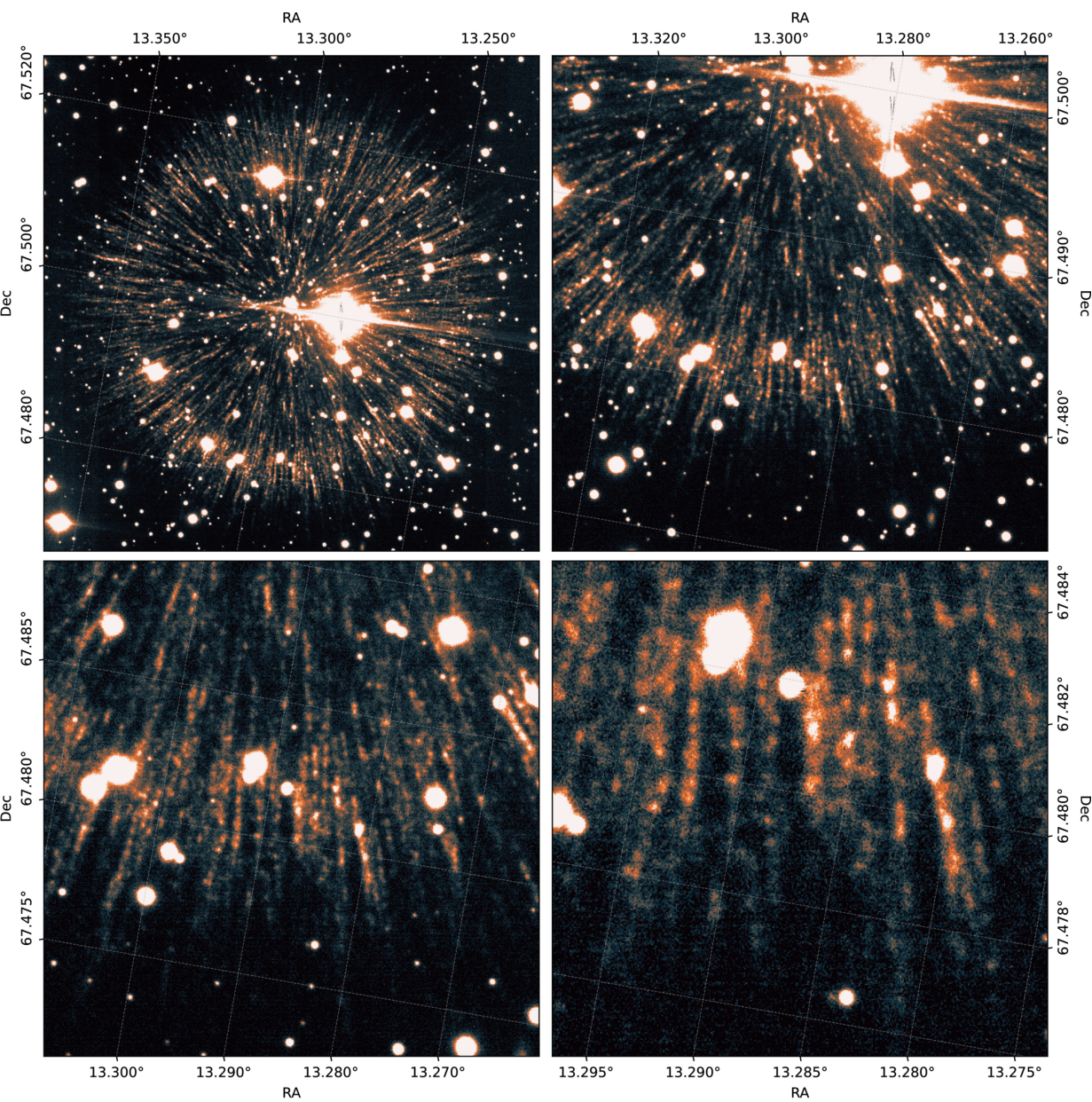
Figure 1. from Tim Cunningham et al 2026 Astrophys. J. 1010 doi:10.3847/1538-4357/ae9cb2 https://dx.doi.org/10.3847/1538-4357/ae9cb2 © 2026. The Author(s). Published by the American Astronomical Society.
