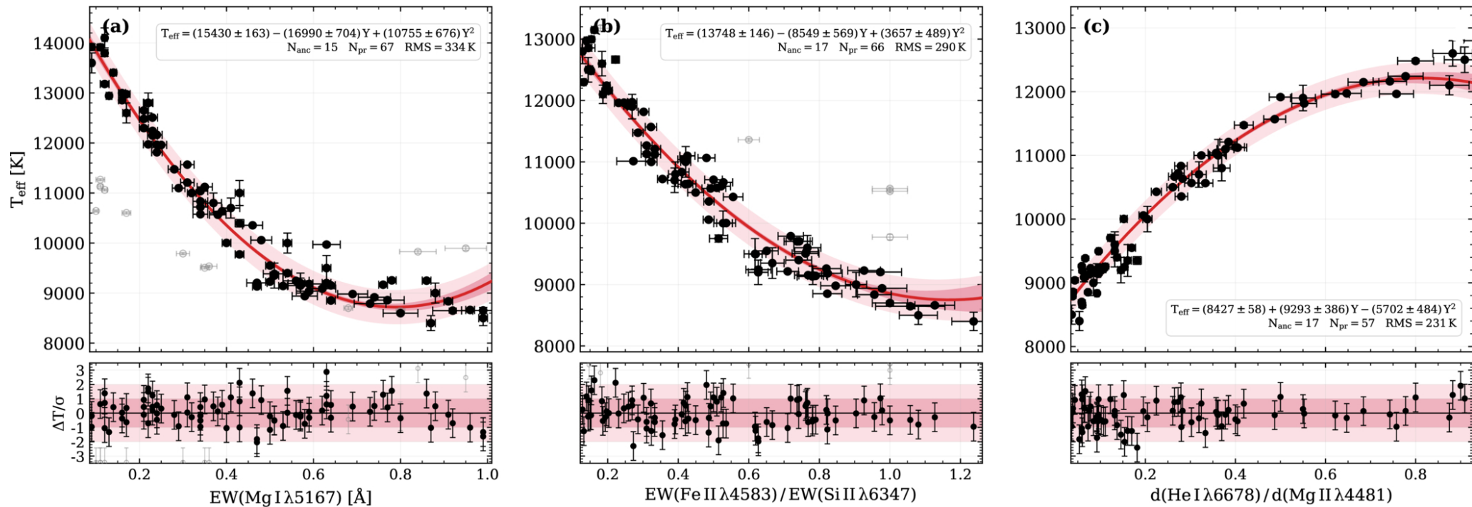
Figure 1. from N. L. Vaidman et al 2026 Astrophys. J. 1010 doi:10.3847/1538-4357/ae9c37 https://dx.doi.org/10.3847/1538-4357/ae9c37 © 2026. The Author(s). Published by the American Astronomical Society.
