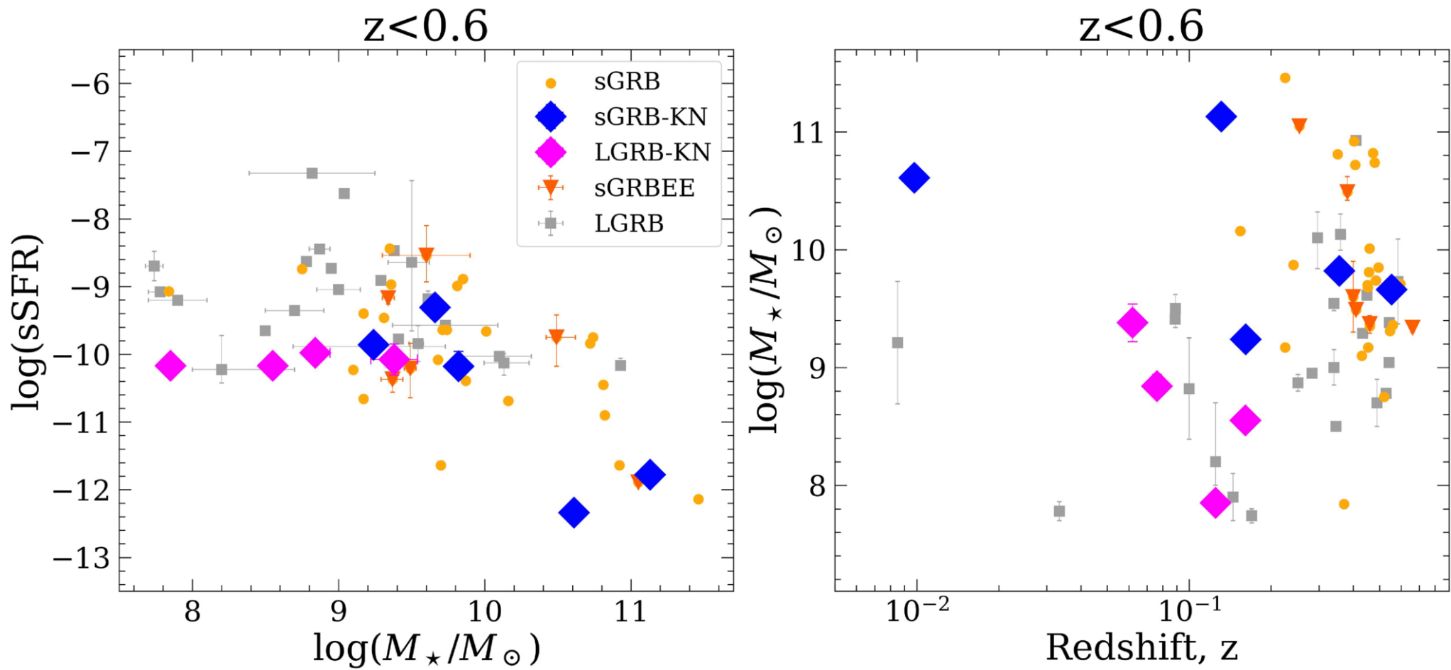
Figure 6. from Hannah Skobe et al 2026 Astrophys. J. 1009 doi:10.3847/1538-4357/ae9c33 https://dx.doi.org/10.3847/1538-4357/ae9c33 © 2026. The Author(s). Published by the American Astronomical Society.
