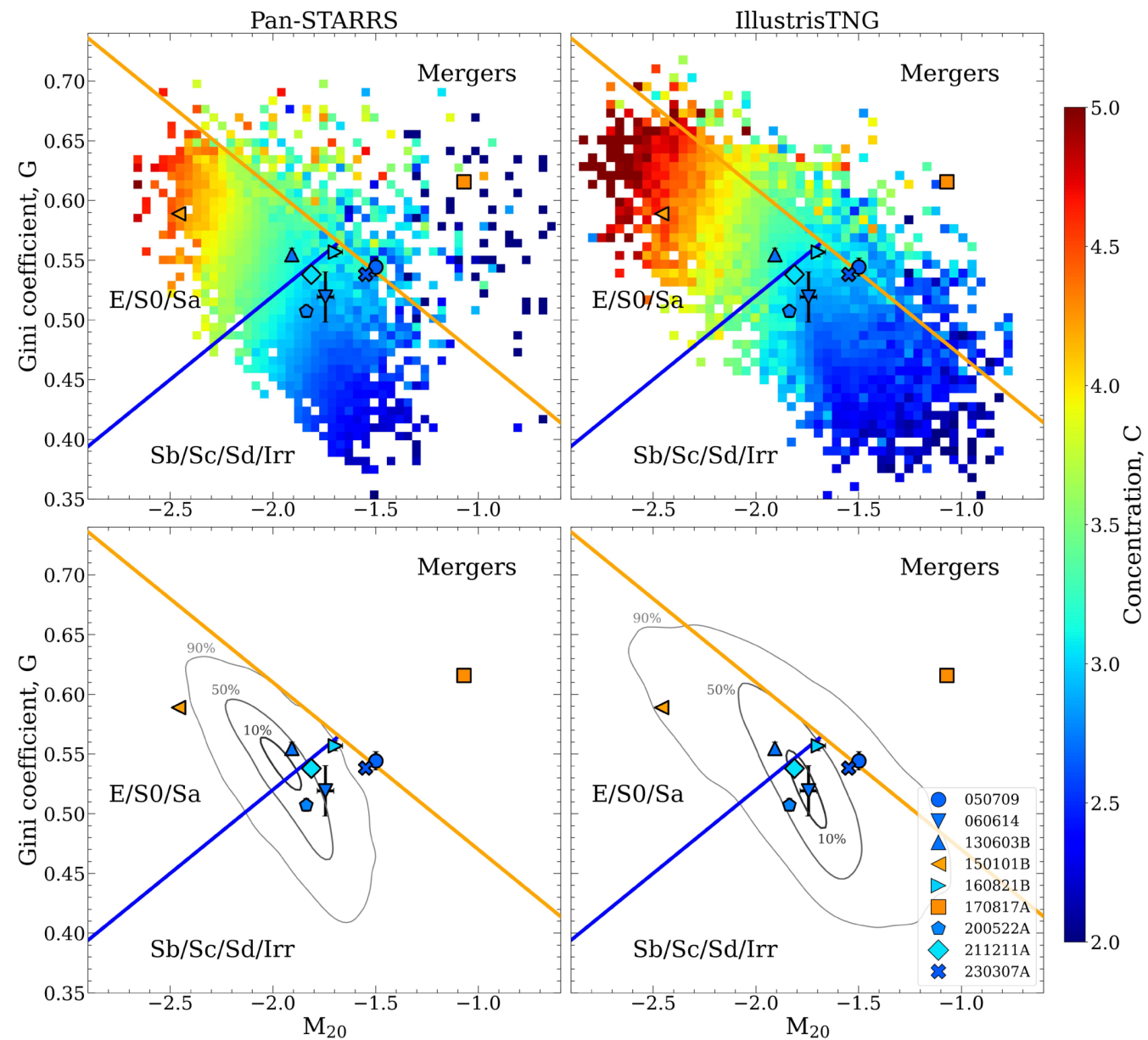
Figure 3. from Hannah Skobe et al 2026 Astrophys. J. 1009 doi:10.3847/1538-4357/ae9c33 https://dx.doi.org/10.3847/1538-4357/ae9c33 © 2026. The Author(s). Published by the American Astronomical Society.
