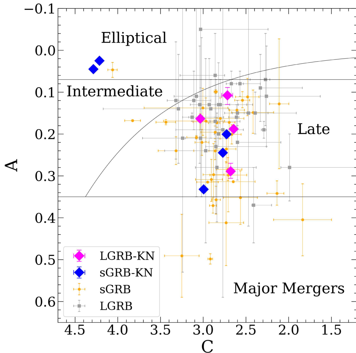
Figure 2. from Hannah Skobe et al 2026 Astrophys. J. 1009 doi:10.3847/1538-4357/ae9c33 https://dx.doi.org/10.3847/1538-4357/ae9c33 © 2026. The Author(s). Published by the American Astronomical Society.
