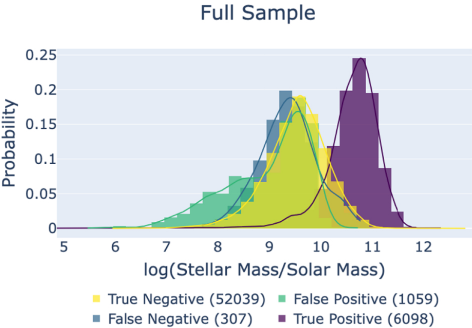
Figure 5. from Alexander Messick and Vivienne Baldassare 2026 Astrophys. J. 1009 doi:10.3847/1538-4357/ae9bc1 https://dx.doi.org/10.3847/1538-4357/ae9bc1 © 2026. The Author(s). Published by the American Astronomical Society.
