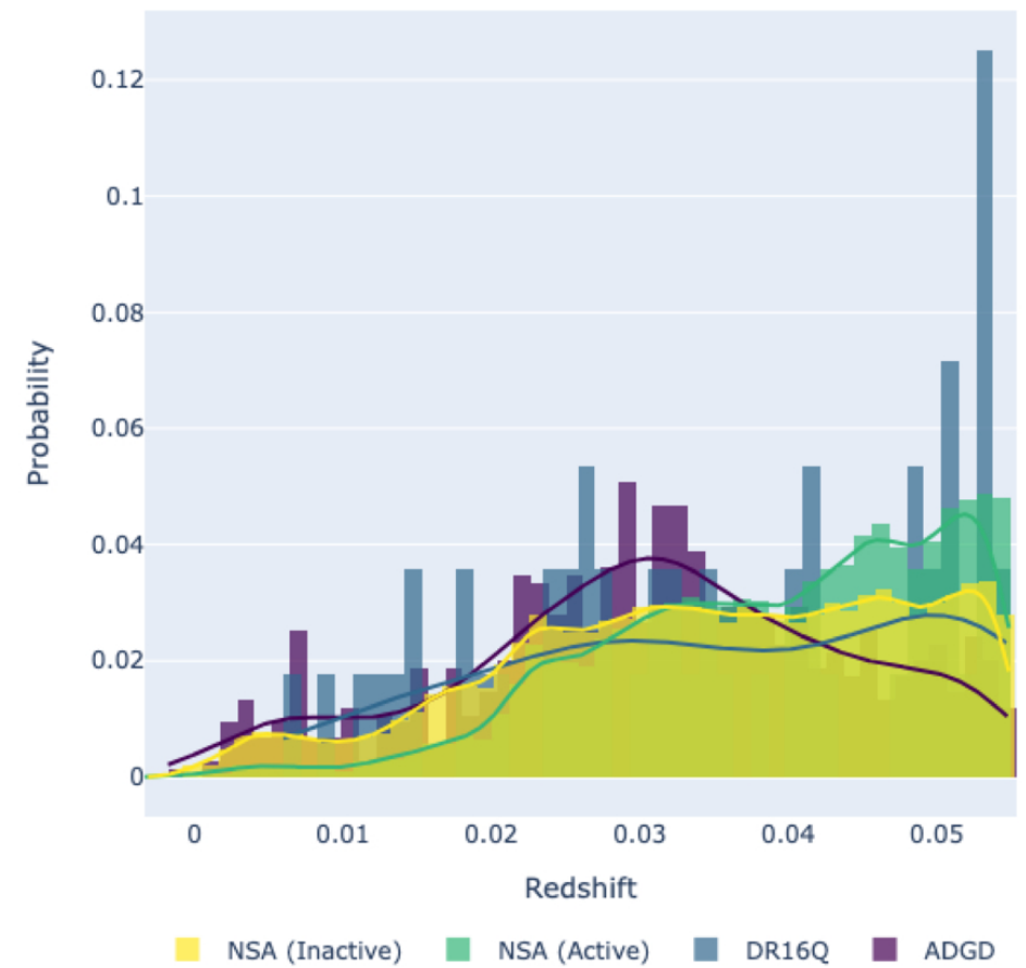
Figure 3. from Alexander Messick and Vivienne Baldassare 2026 Astrophys. J. 1009 doi:10.3847/1538-4357/ae9bc1 https://dx.doi.org/10.3847/1538-4357/ae9bc1 © 2026. The Author(s). Published by the American Astronomical Society.
