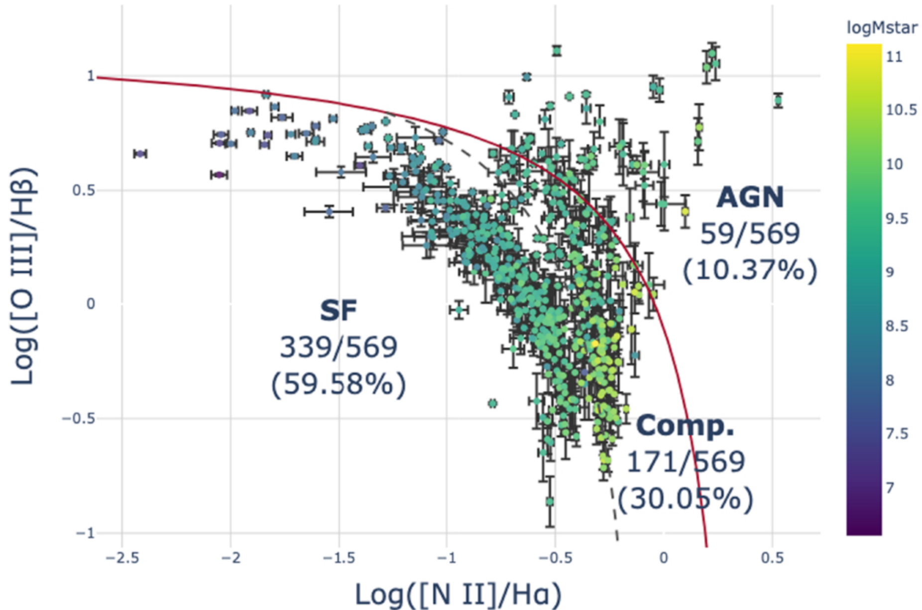
Figure 1. from Alexander Messick and Vivienne Baldassare 2026 Astrophys. J. 1009 doi:10.3847/1538-4357/ae9bc1 https://dx.doi.org/10.3847/1538-4357/ae9bc1 © 2026. The Author(s). Published by the American Astronomical Society.
