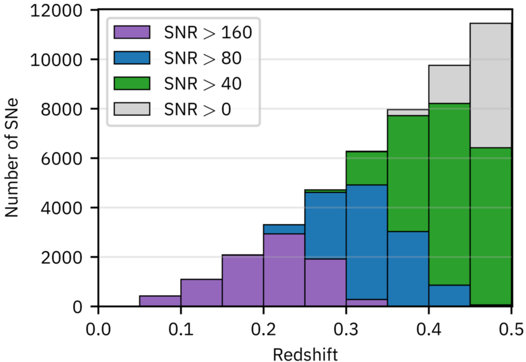
Figure 7. from Jannik Truong et al 2026 Astrophys. J. 1009 doi:10.3847/1538-4357/ae9a98 https://dx.doi.org/10.3847/1538-4357/ae9a98 © 2026. The Author(s). Published by the American Astronomical Society.
