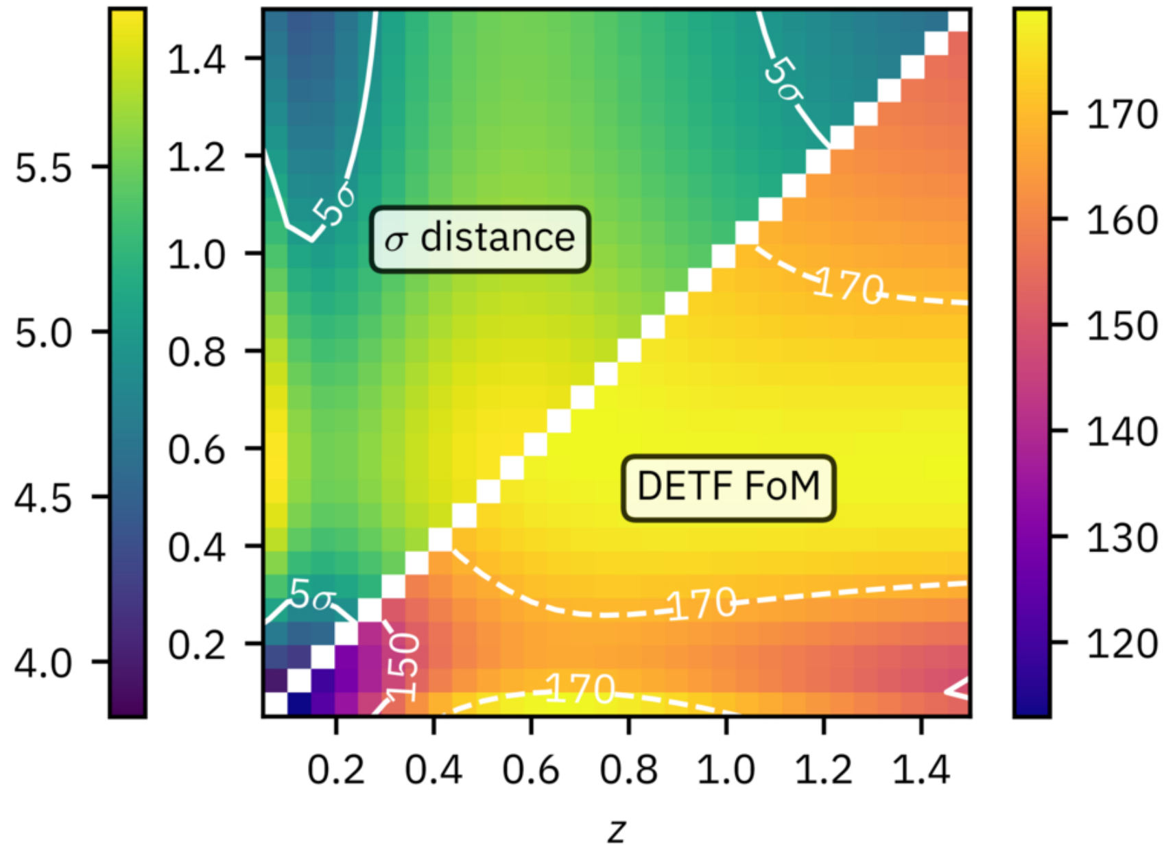
Figure 5. from Jannik Truong et al 2026 Astrophys. J. 1009 doi:10.3847/1538-4357/ae9a98 https://dx.doi.org/10.3847/1538-4357/ae9a98 © 2026. The Author(s). Published by the American Astronomical Society.
