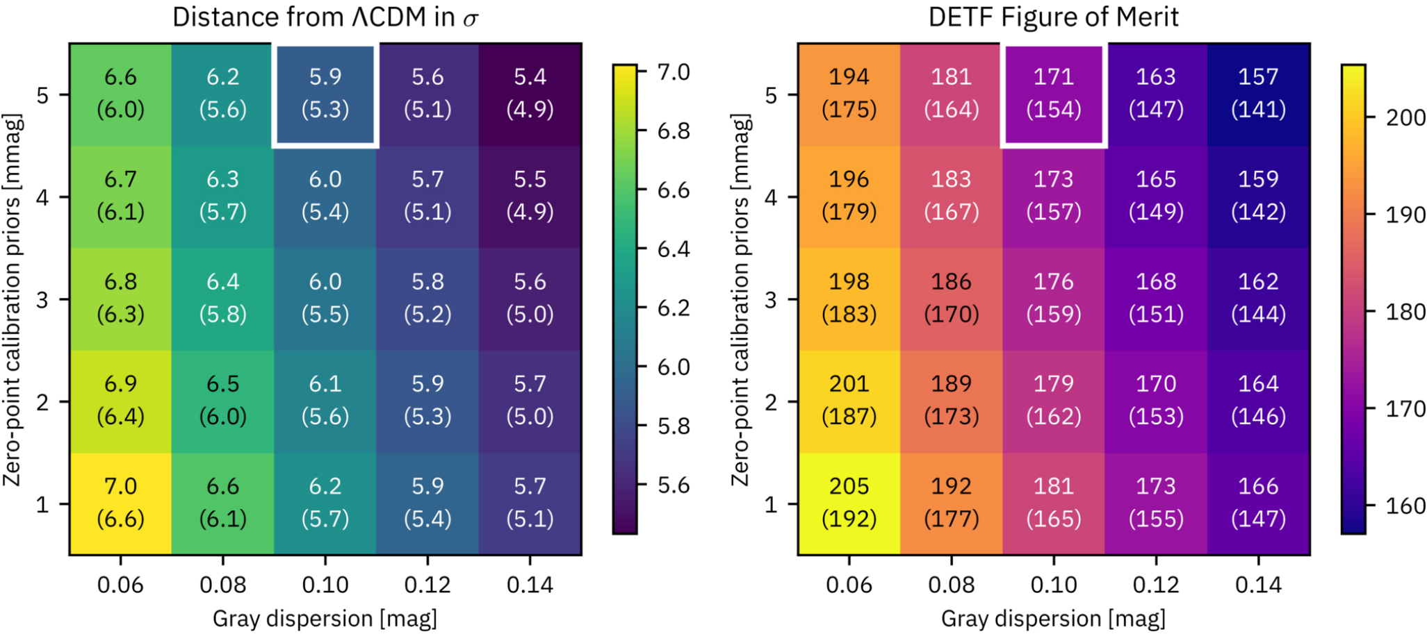
Figure 19. from Jannik Truong et al 2026 Astrophys. J. 1009 doi:10.3847/1538-4357/ae9a98 https://dx.doi.org/10.3847/1538-4357/ae9a98 © 2026. The Author(s). Published by the American Astronomical Society.
