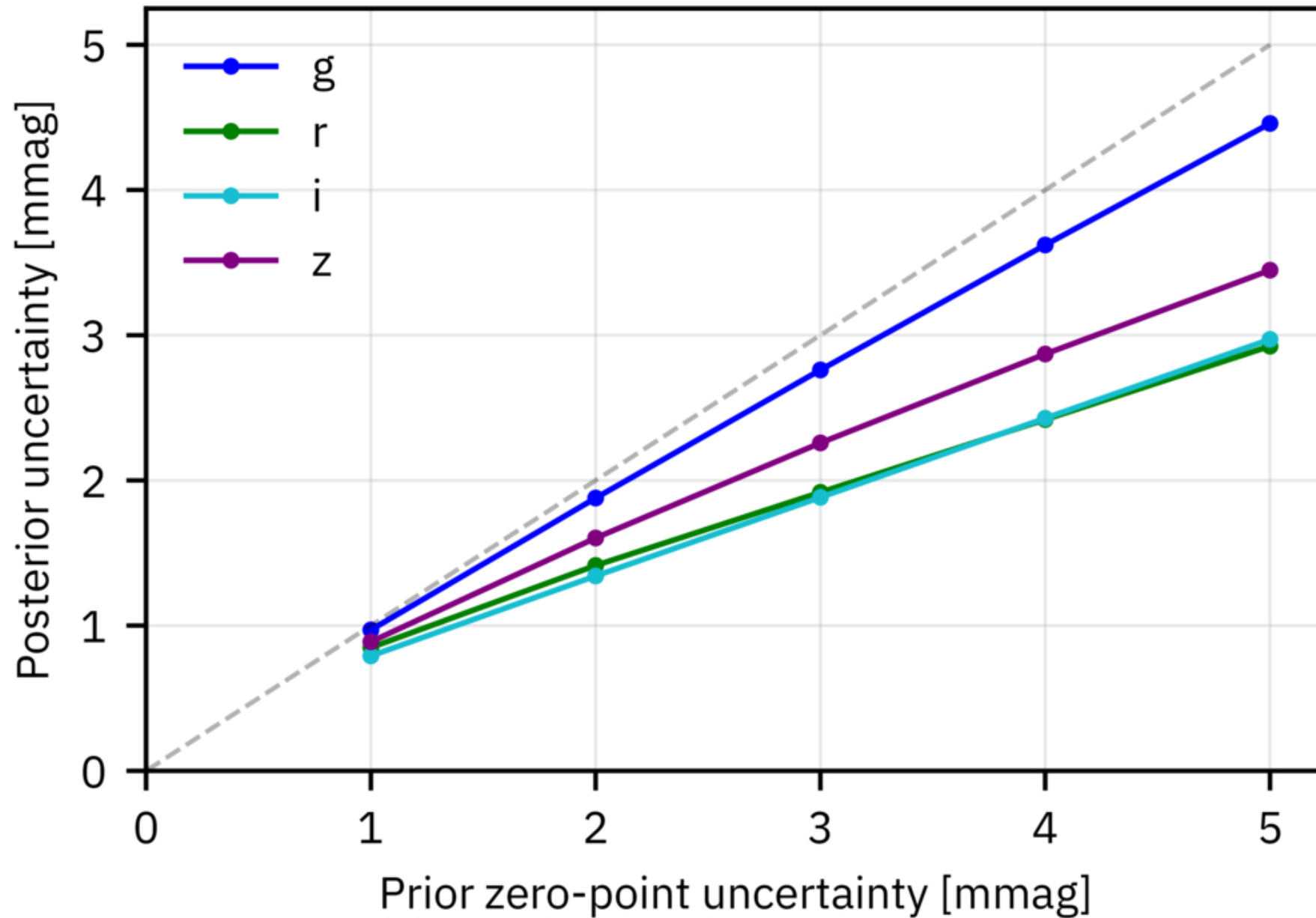
Figure 18. from Jannik Truong et al 2026 Astrophys. J. 1009 doi:10.3847/1538-4357/ae9a98 https://dx.doi.org/10.3847/1538-4357/ae9a98 © 2026. The Author(s). Published by the American Astronomical Society.
