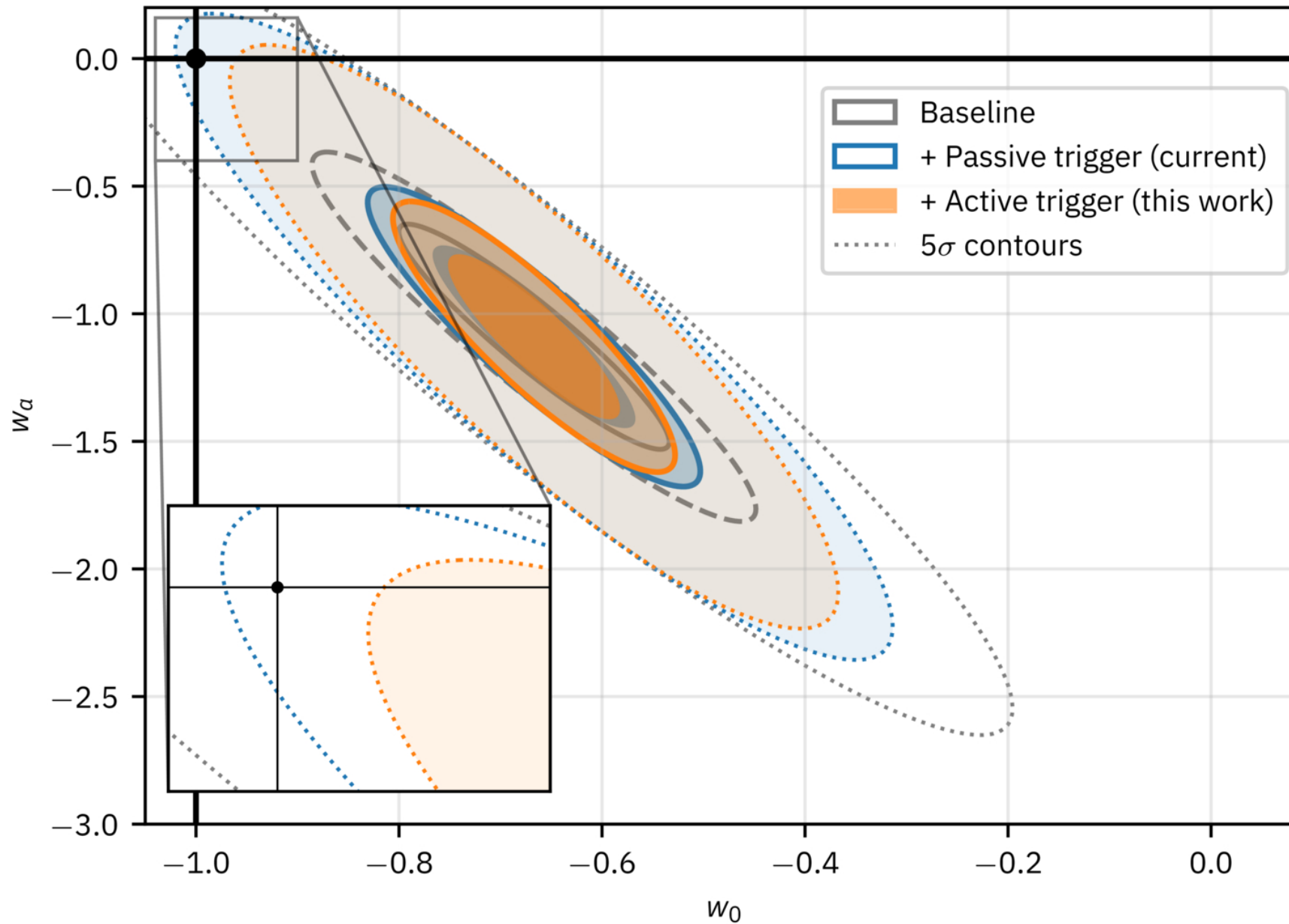
Figure 15. from Jannik Truong et al 2026 Astrophys. J. 1009 doi:10.3847/1538-4357/ae9a98 https://dx.doi.org/10.3847/1538-4357/ae9a98 © 2026. The Author(s). Published by the American Astronomical Society.
