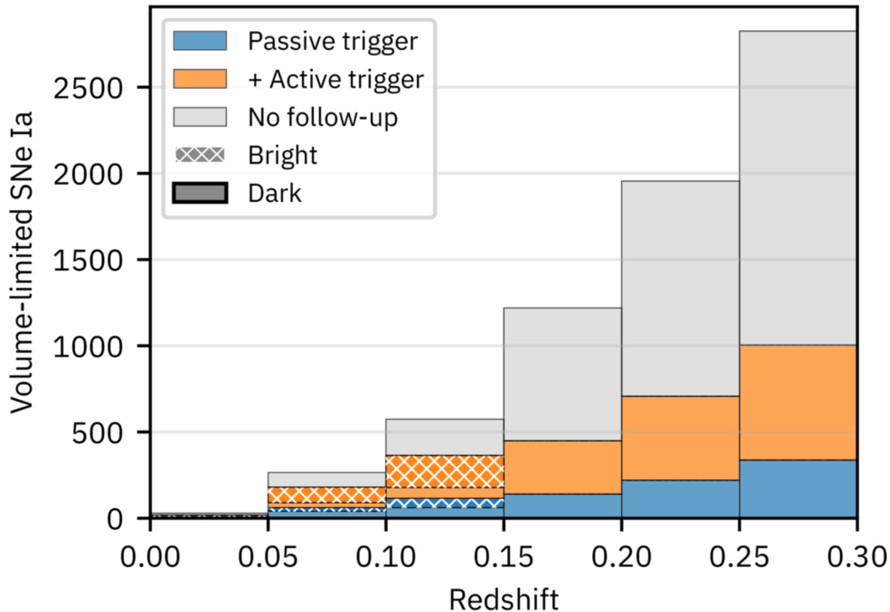
Figure 12. from Jannik Truong et al 2026 Astrophys. J. 1009 doi:10.3847/1538-4357/ae9a98 https://dx.doi.org/10.3847/1538-4357/ae9a98 © 2026. The Author(s). Published by the American Astronomical Society.
