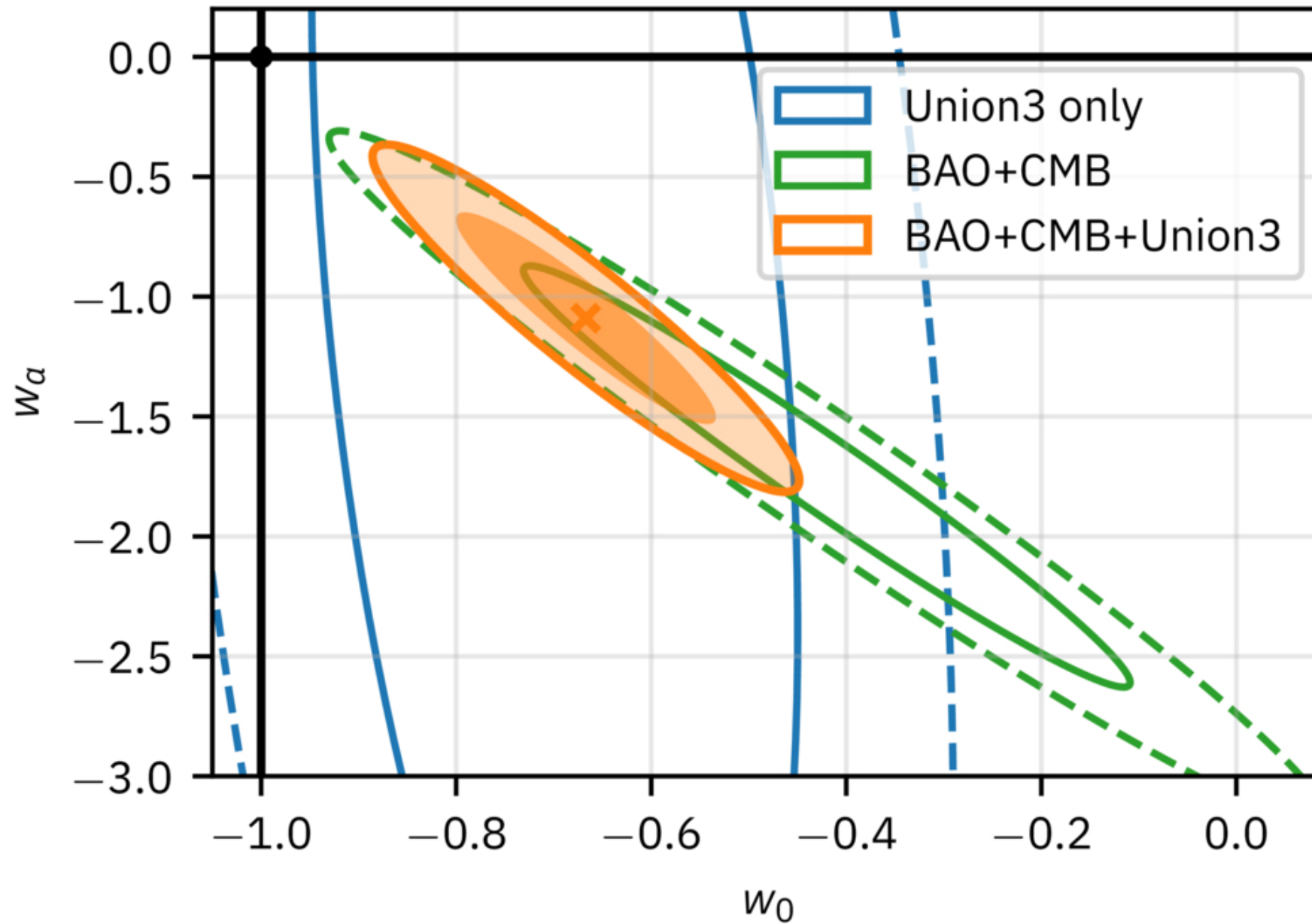
Figure 1. from Jannik Truong et al 2026 Astrophys. J. 1009 doi:10.3847/1538-4357/ae9a98 https://dx.doi.org/10.3847/1538-4357/ae9a98 © 2026. The Author(s). Published by the American Astronomical Society.
