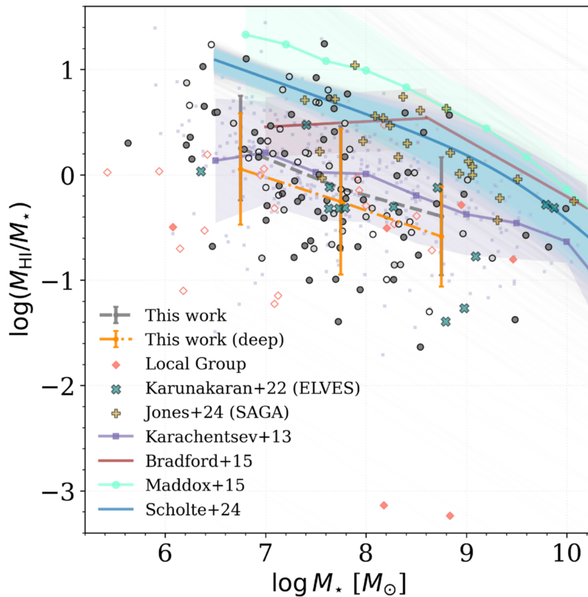
Figure 6. from Jingyao Zhu et al 2026 Astrophys. J. 1009 doi:10.3847/1538-4357/ae9a95 https://dx.doi.org/10.3847/1538-4357/ae9a95 © 2026. The Author(s). Published by the American Astronomical Society.
