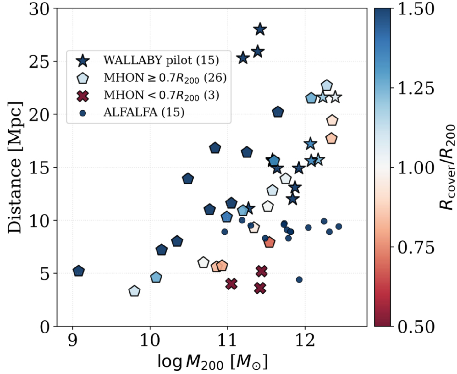
Figure 1. from Jingyao Zhu et al 2026 Astrophys. J. 1009 doi:10.3847/1538-4357/ae9a95 https://dx.doi.org/10.3847/1538-4357/ae9a95 © 2026. The Author(s). Published by the American Astronomical Society.
