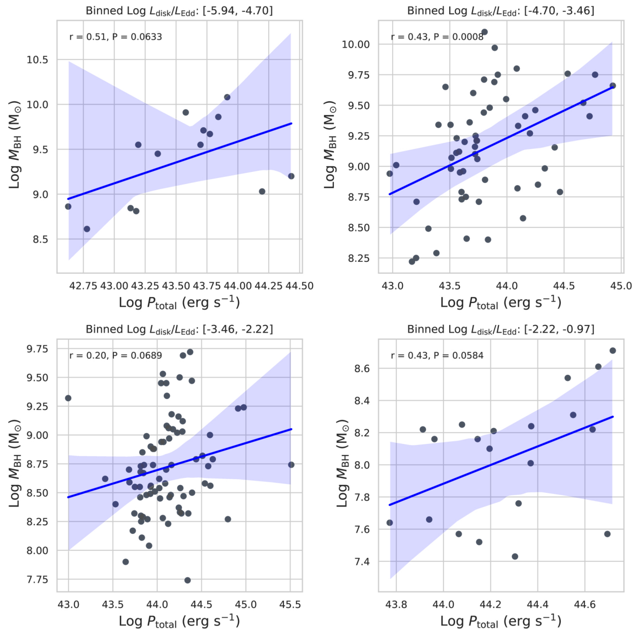
Figure 9. from Dingrong Xiong et al 2026 Astrophys. J. 1009 doi:10.3847/1538-4357/ae9a92 https://dx.doi.org/10.3847/1538-4357/ae9a92
