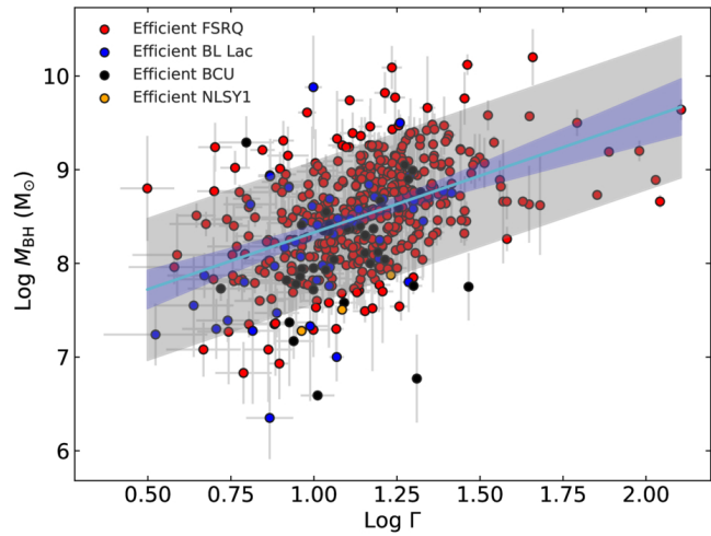
(c) Black hole mass versus bulk Lorentz factor in radiatively efficient AGNs
