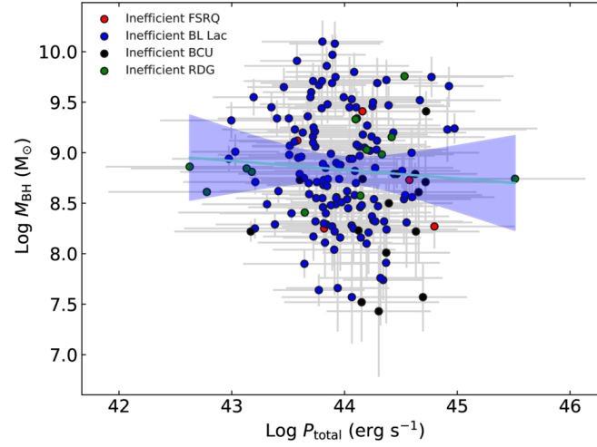
(b) Black hole mass versus total jet power in radiatively inefficient AGNs
