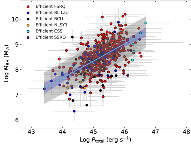
(a) Black hole mass versus total jet power in radiatively efficient AGNs
