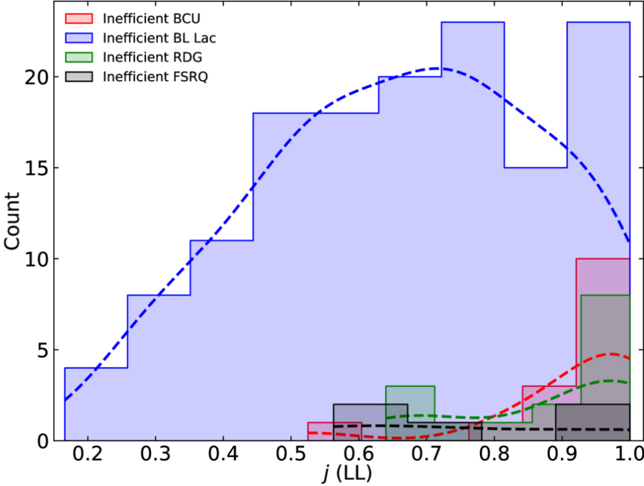
(b) Radiatively inefficient AGNs
