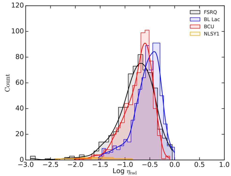
(b) Jet radiative efficiency
