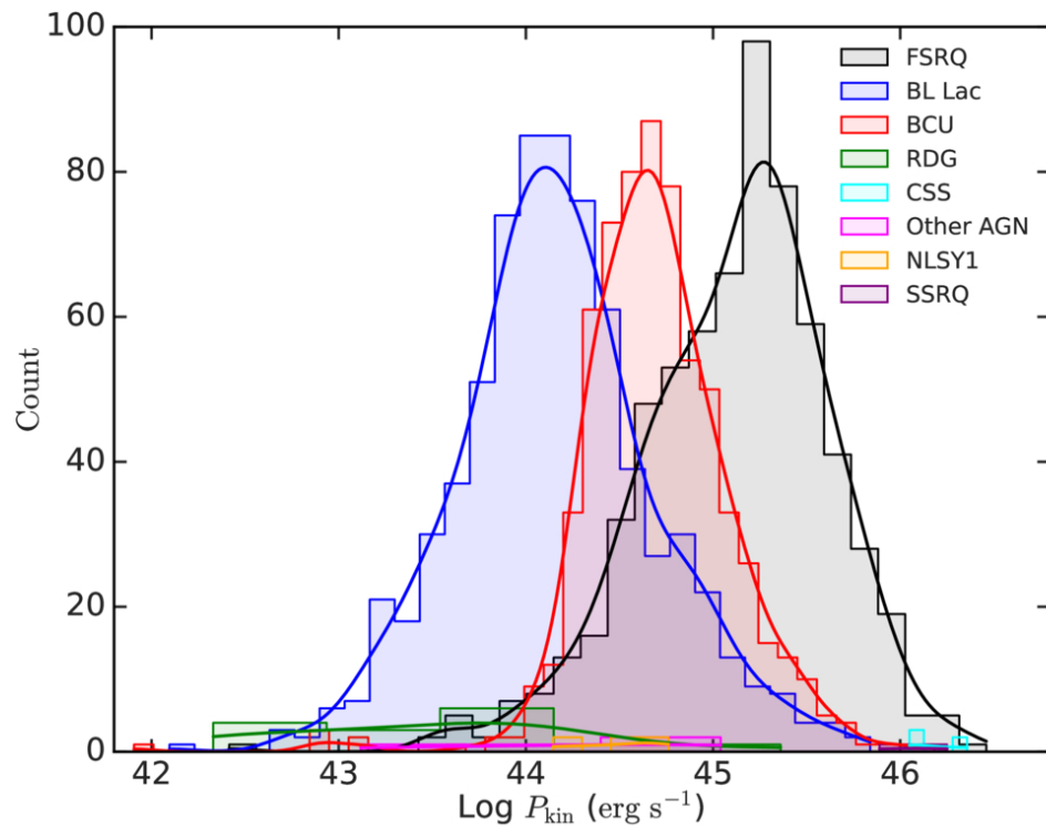
Figure 5. from Dingrong Xiong et al 2026 Astrophys. J. 1009 doi:10.3847/1538-4357/ae9a92 https://dx.doi.org/10.3847/1538-4357/ae9a92 © 2026. The Author(s). Published by the American Astronomical Society.
