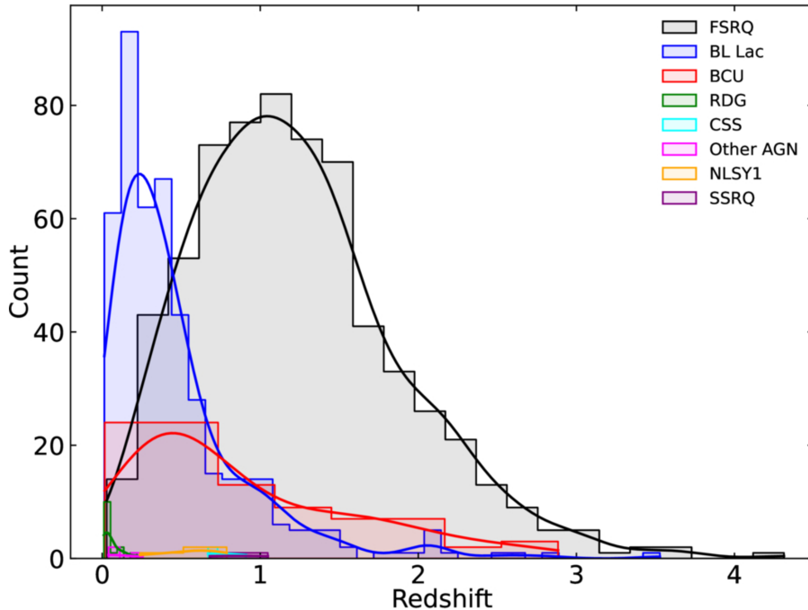
Figure 4. from Dingrong Xiong et al 2026 Astrophys. J. 1009 doi:10.3847/1538-4357/ae9a92 https://dx.doi.org/10.3847/1538-4357/ae9a92 © 2026. The Author(s). Published by the American Astronomical Society.
